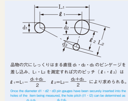
～穴のピッチ測定～ Hole Pitch Measurement
