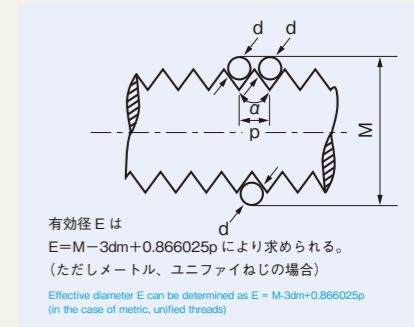
～ねじの有効径測定(三針法)～ Thread Effective Diameter Measurement (3-pin method)
